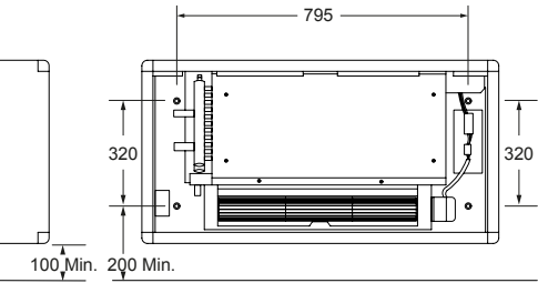
Minimum floor clearance/mounting centers
