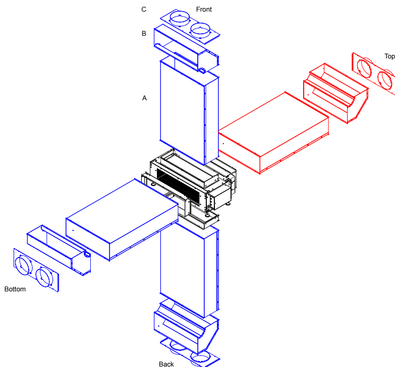
Exploded diagram with base unit shown in centre laying on its back, all other parts available separately
