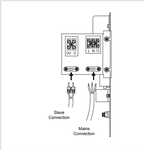
Remote / flush control options (electrical connection moved adjacent to wiring panel)
