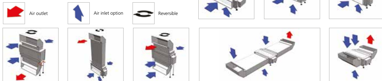
Suspended with spigots application
